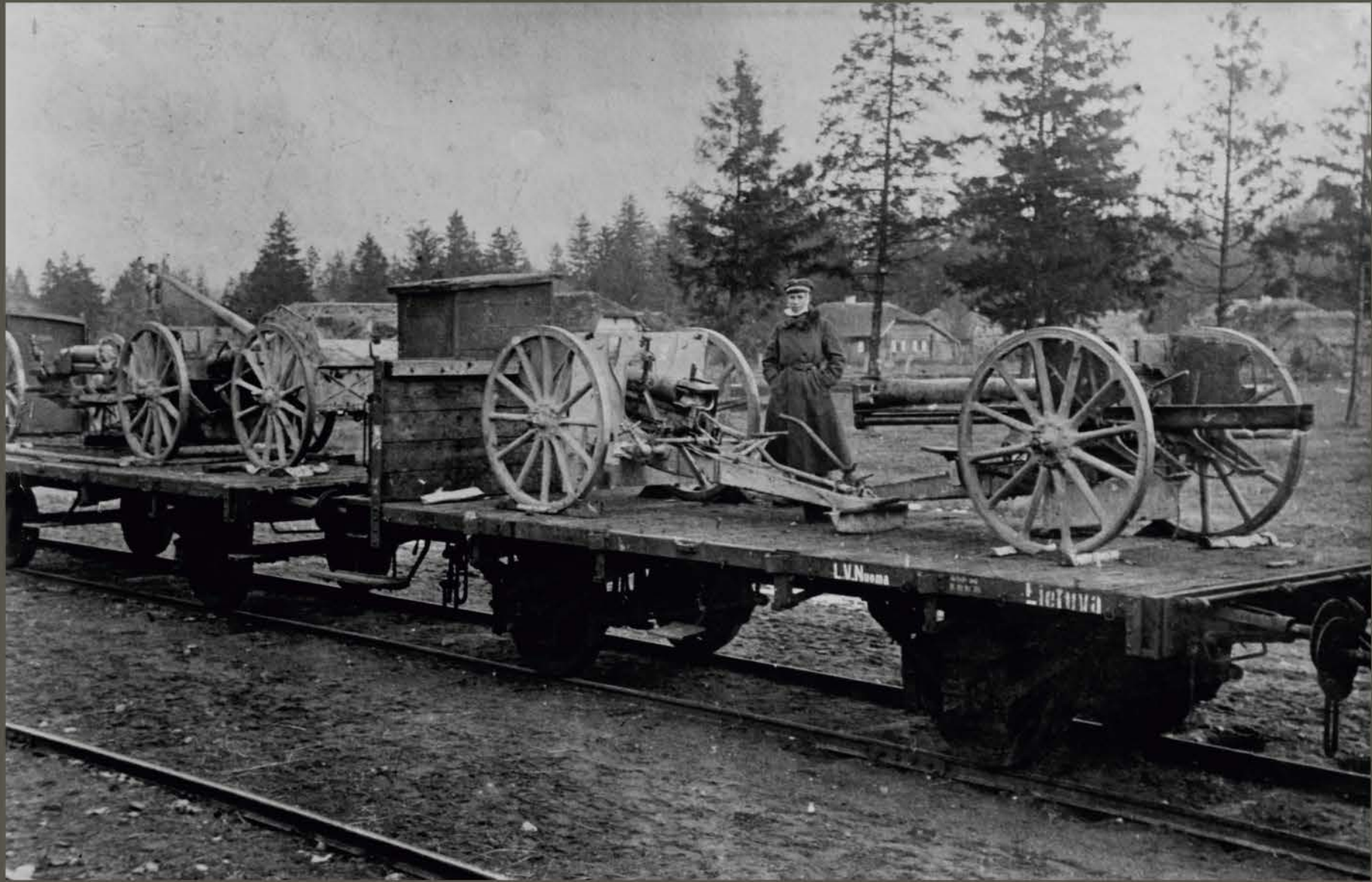
77 mm kalibro 96 N. A modelio lauko patrankos Lietuvos kariuomenės atimtos iš bermontininkų Radviliškio geležinkelio stoties. 1919 m. 77 mm caliber 96 N. Model A field guns, which were taken away from the Bermontians by the Lithuanian Armed Forces. Radviliškis Railway Station. 1919
